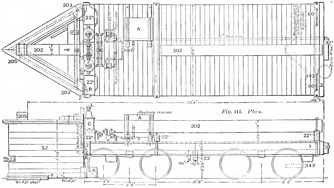
Fig. 415. Side Elevation.
